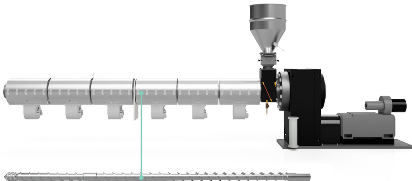
(Shown above: Wilmington Machinery 6" Extruder Assembly with 6", 30:1 L/D Feed Screw)
